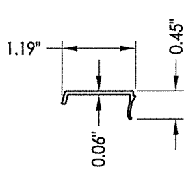
3 GLAZING BEAD 8570-356-D57
