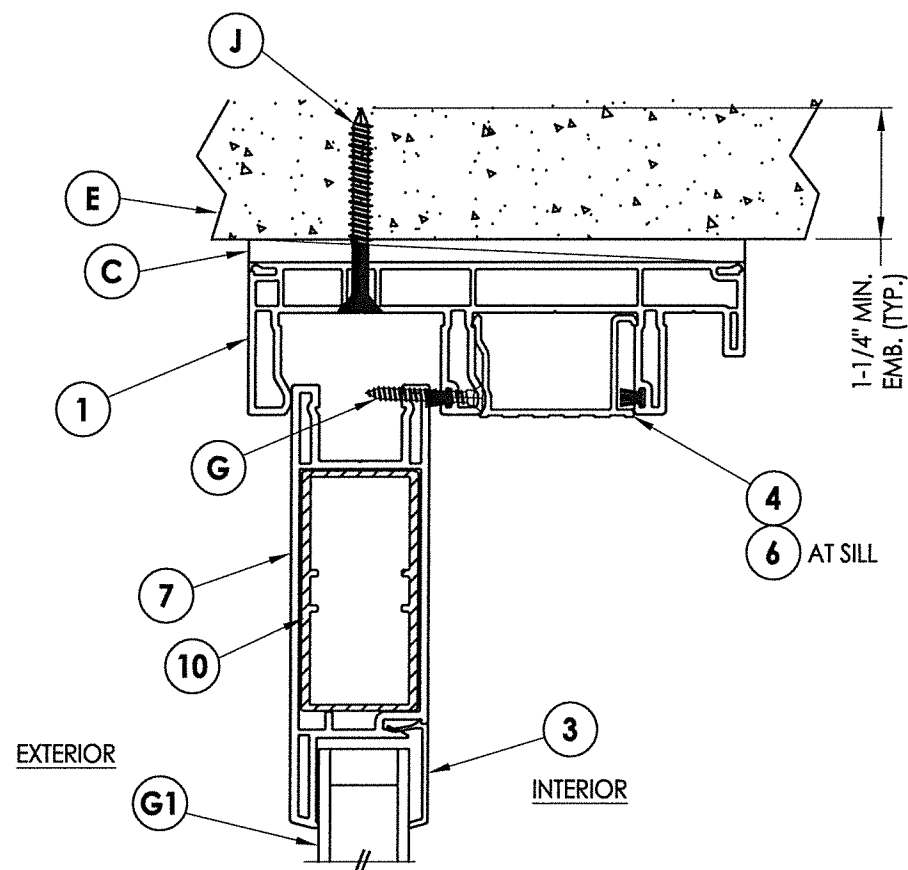
3 VERTICAL CROSS SECTION 3 Direct to Masonry Construction
