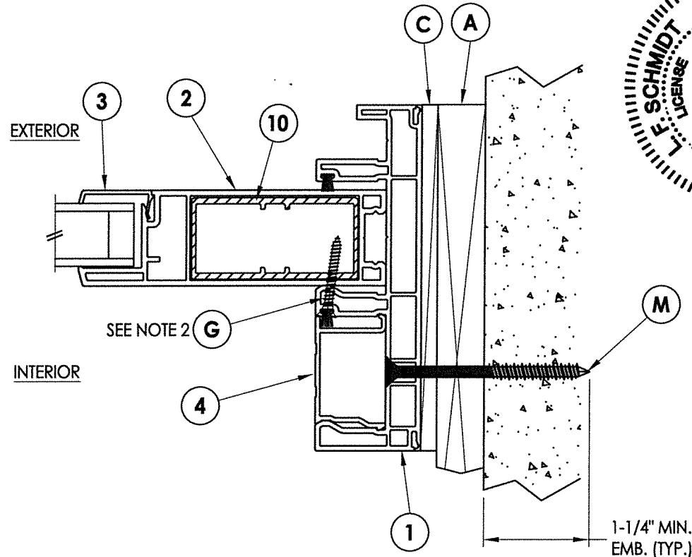
2 HORIZONTAL CROSS SECTION 2 1X Buck Masonry Construction
